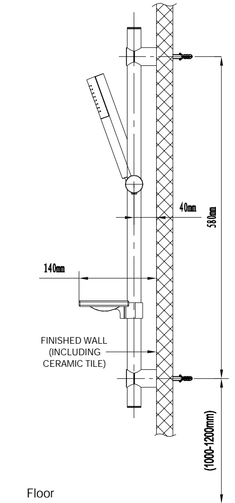
Handheld Shower & Slide Bar And Soap Dish Trim Kit Models: A805-30
